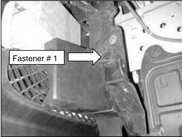
i. Remove the air duct shown by removing the three plastic fasteners holding it in place. (See next page)
