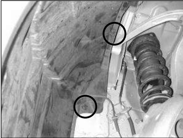
g. From inside the wheel well, remove the two plastic fasteners shown in the picture.
