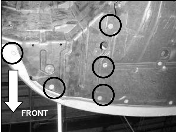
f. From underneath the car, remove the bolts circled in the picture.
