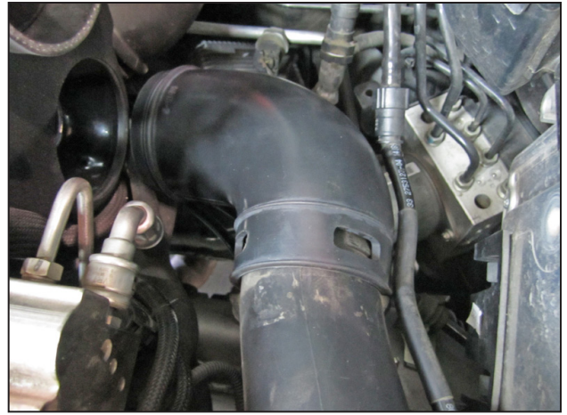
s. Install the oval end of the rubber elbow intake coupler (5-1058) over the outlet of the stock plastic intake tube. Fully seat the coupler until the 4 plastic lock tabs fit into the 4 slots in rubber elbow coupler.
