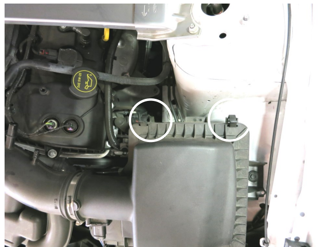
d. Unlatch the two clips securing the upper air box to the lower air box.
