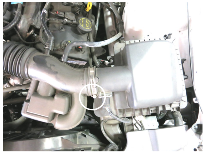
b. Loosen the hose clamp at the air box outlet.
