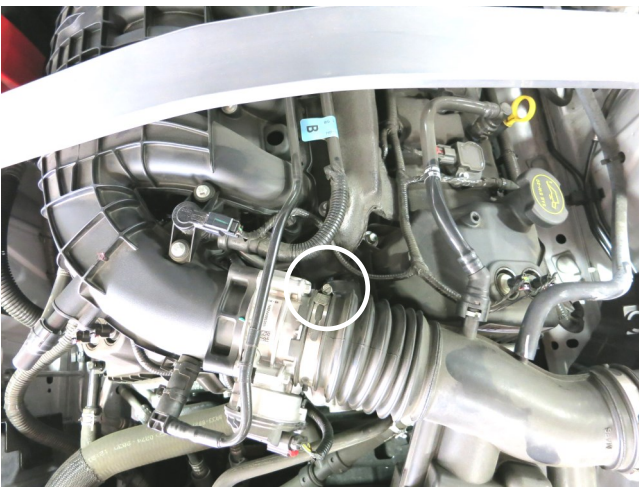
a. Loosen the hose clamp at the throttle body.
