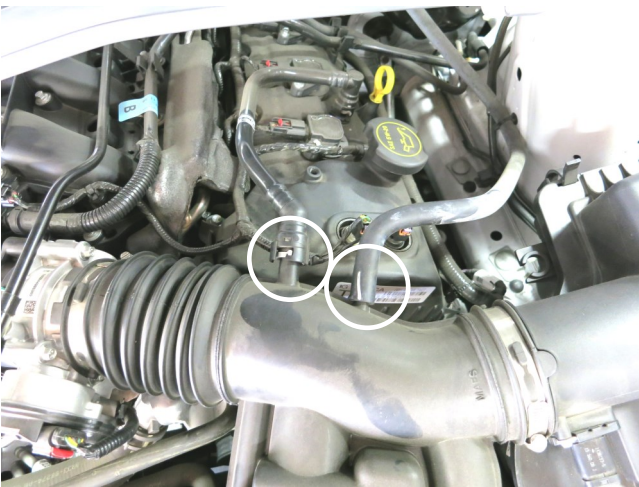
c. Release the pressure on the gray tab and pull the two vent lines from the stock intake tube. Note: Some models may not be equipped with an EVAP vent line.
