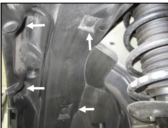
O. Remove the four front upper clips securing the splash shield.
