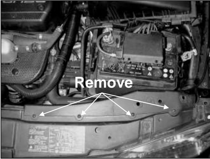
c. Remove the four screws along the top of the radiator support. Remove the two plastic covers.
