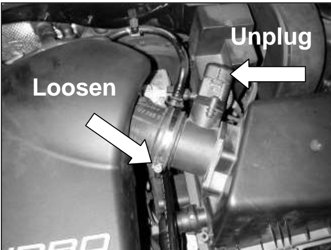
e. Unplug the wire harness from the MAF sensor. Loosen the hose clamp on the engine side of the MAF sensor. Pull the rubber tube off of the MAF sensor.
