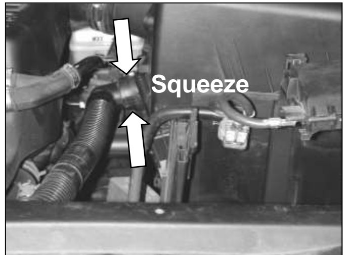
f. Squeeze the top and bottom of the breather hose. Pull the breather hose clear from the air box. NOTE: N/A for diesel models.
