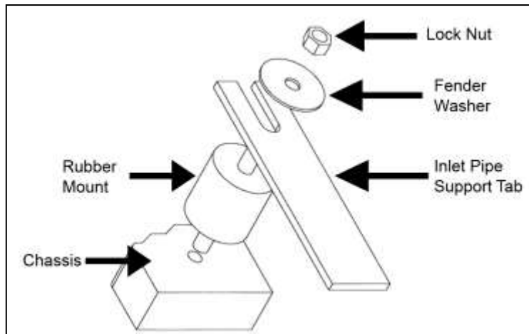
o. Align the mounting bracket to the rubber mount installed in step 3b. See diagram below for proper assembly.
