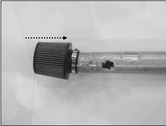
l. Attach the air filter element to the end of the inlet pipe. Secure with hose clamp.
